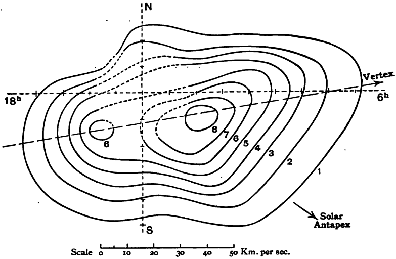
FIG. 21.—Curves of Equal Frequency of Velocity.
